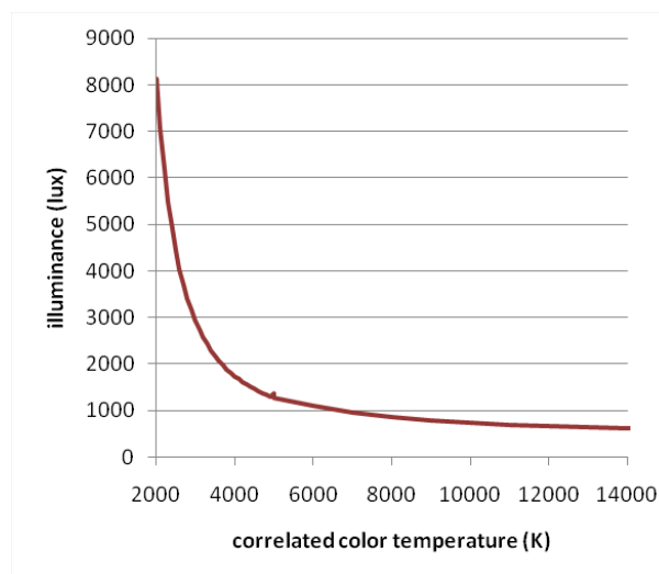
Figure 1: Estimate of the illuminance level where EB = 1 W/m^2 , border between RG 1 ( t_{max} > 100 s) and RG 2 ( t_{max} < 100 s) in the small source regime, as a function of CCT
